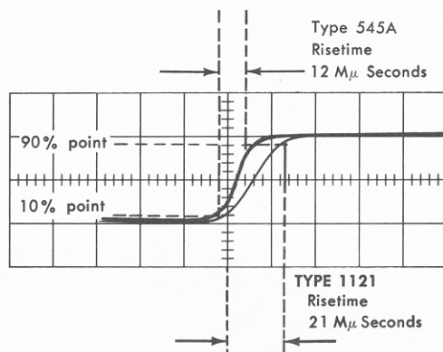
Fig. 1-1. Comparison of vertical risetimes of the Type 1121 and Type 545A Oscilloscope.
